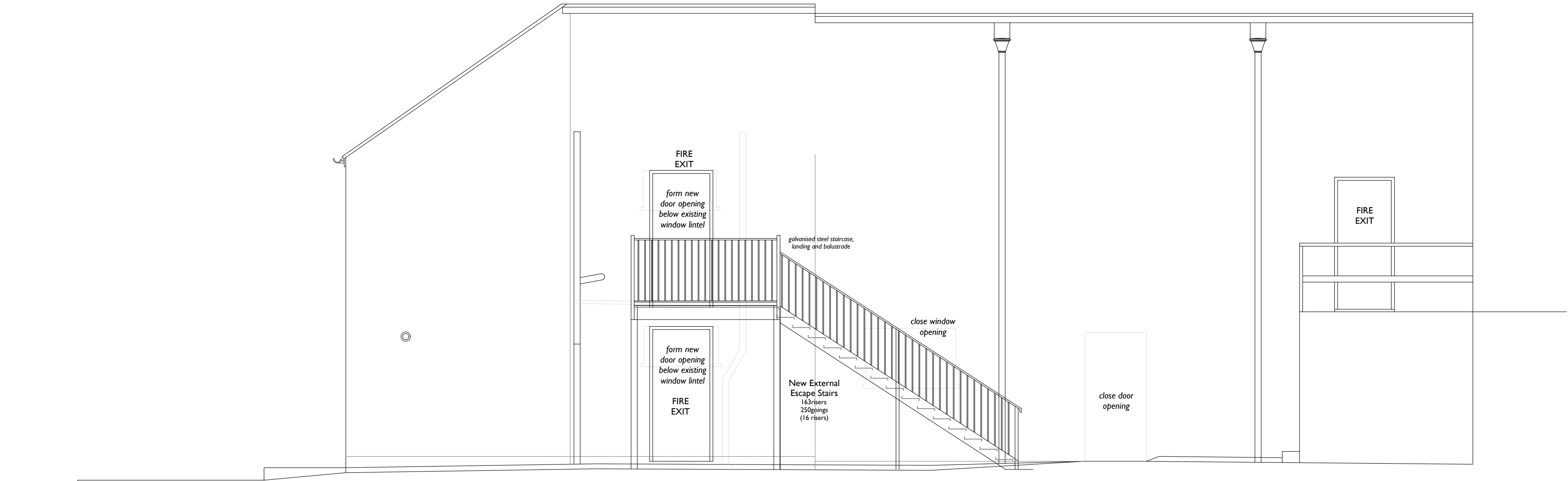
Proposed Side Elevation North East
