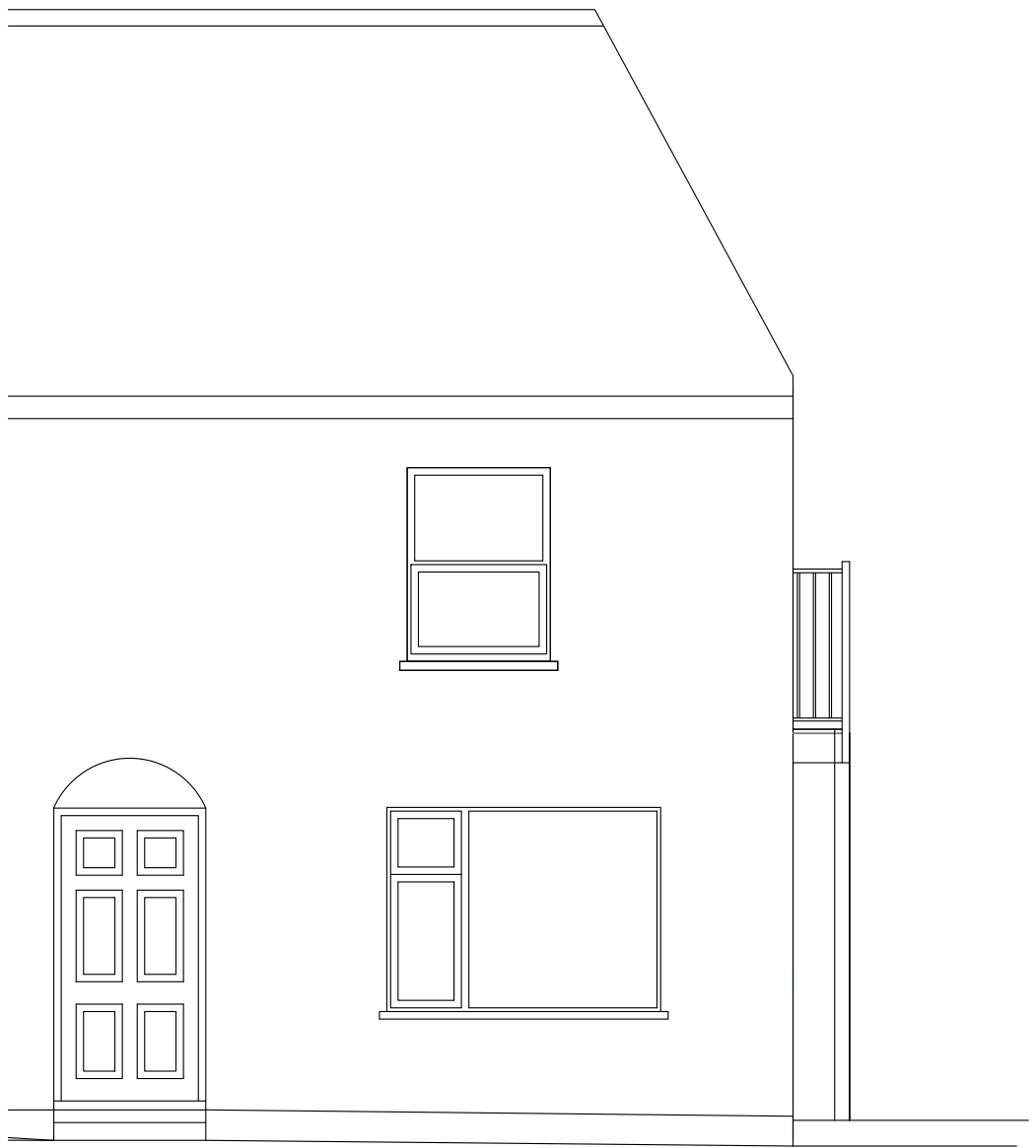
Proposed Front Elevation South East
