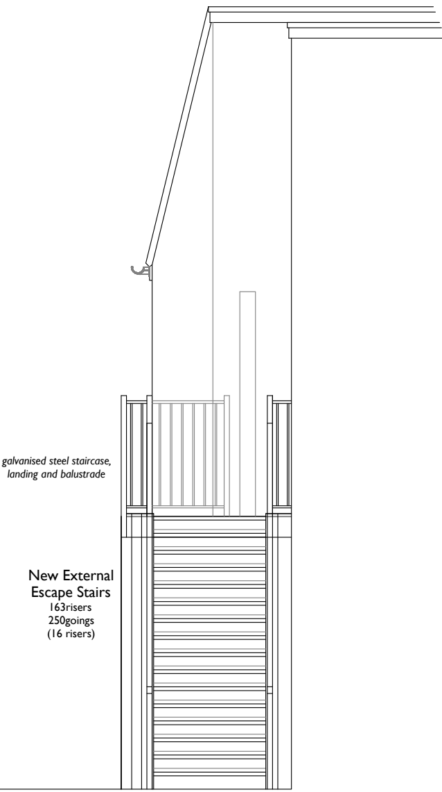
Proposed Rear Elevation North West
